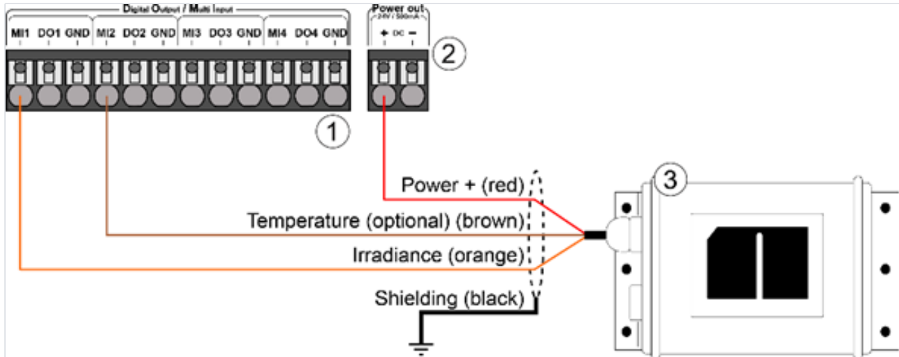
Si-V-010, Si-V-010-T, Si-I-420, Si-I-420-T (analog interface): Sensor connection
