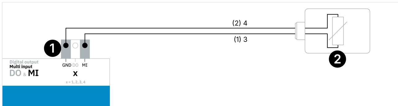
PT1000 sensor in the housing
