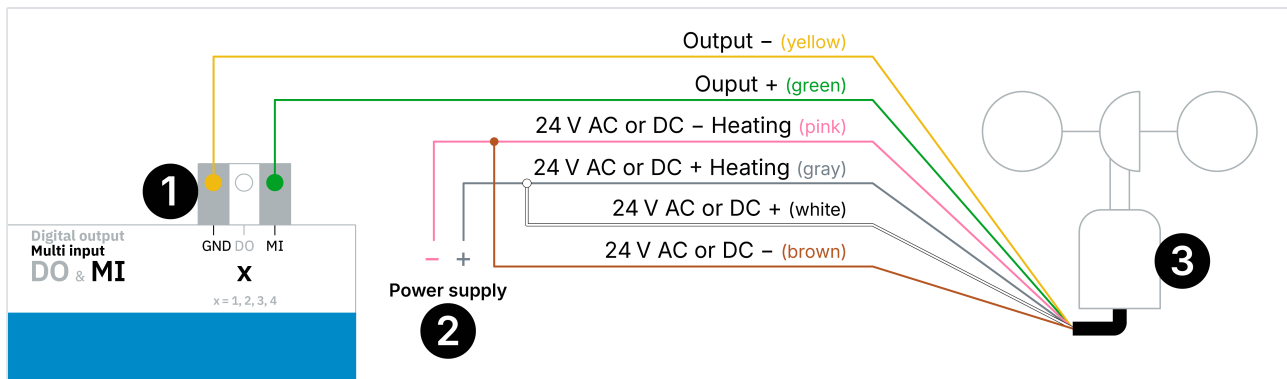
mc compact wind speed sensor: Sensor connection
