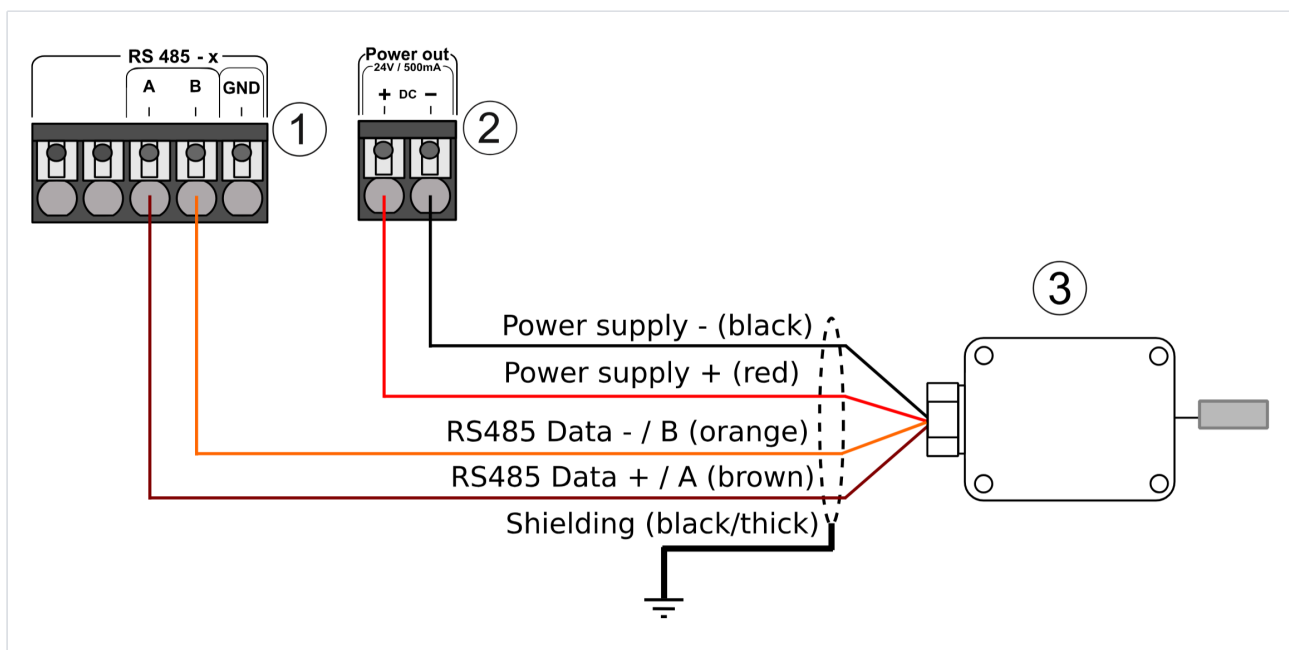
Tm-RS485-MB module temperature sensor (Modbus RTU): Sensor connection
