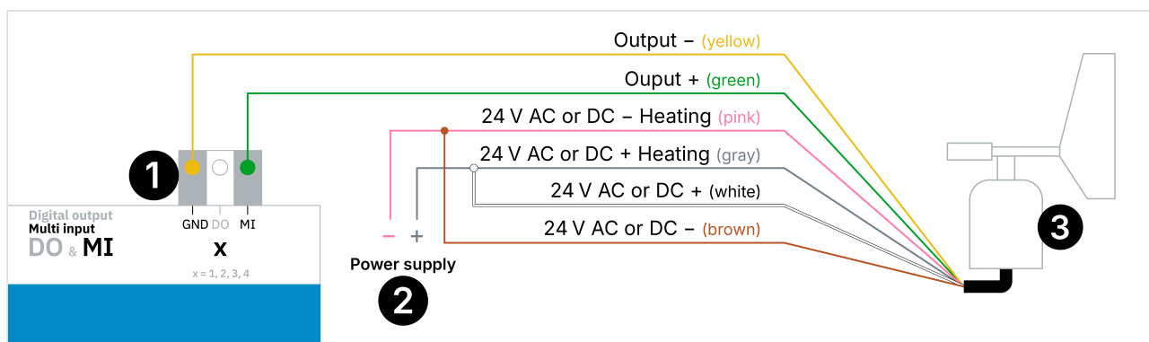
mc compact wind direction sensor: Sensor connection
