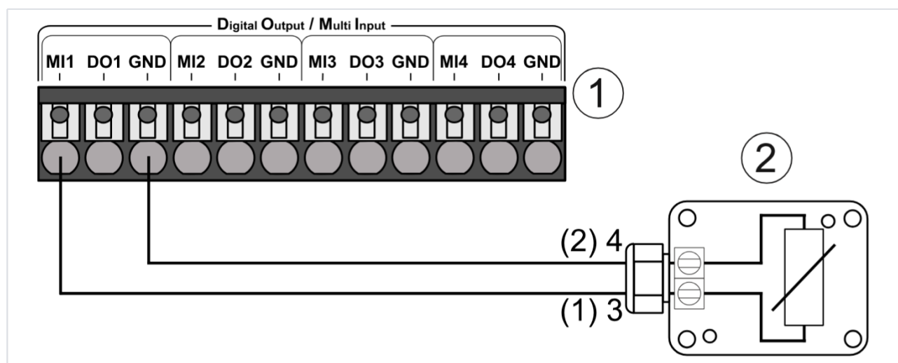
PT1000 sensor in the housing
