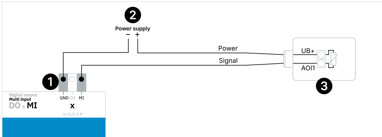
Thermokon AGS55+ ambient temperature sensor: Sensor connection
