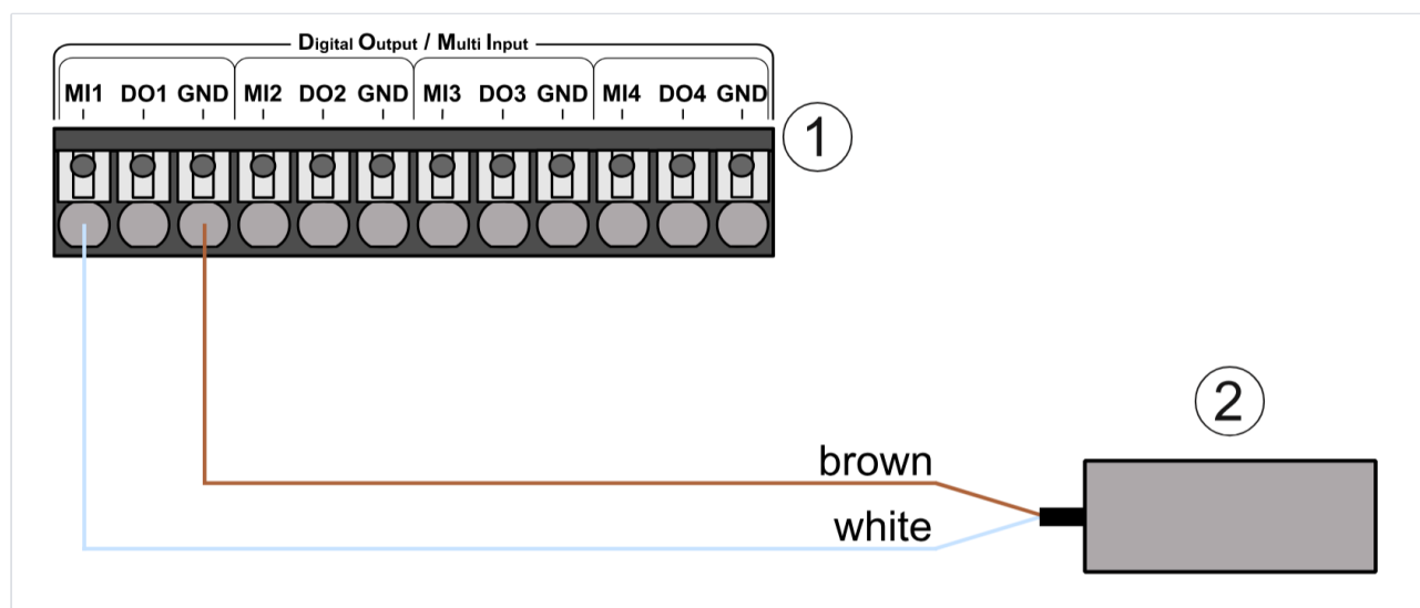
PT1000 adhesive sensor: Sensor connection
