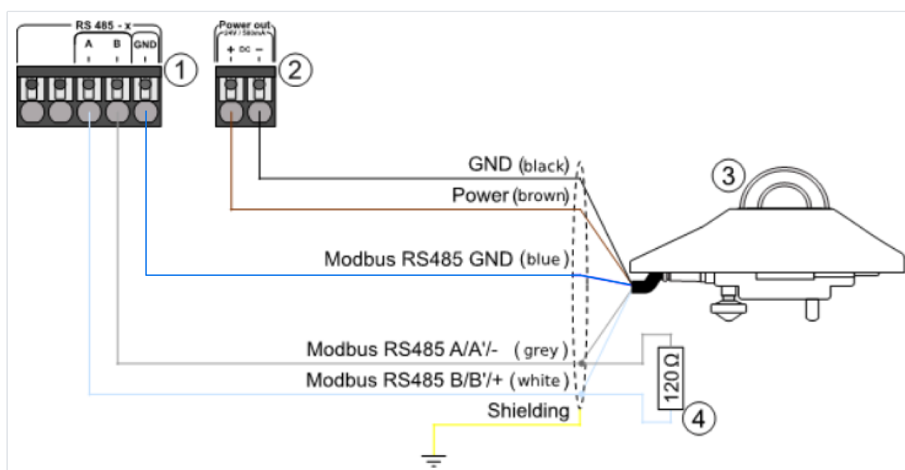
Hukseflux SR200-D1, SR300-D1, SR05-D1A (Modbus RTU): Sensor connection
