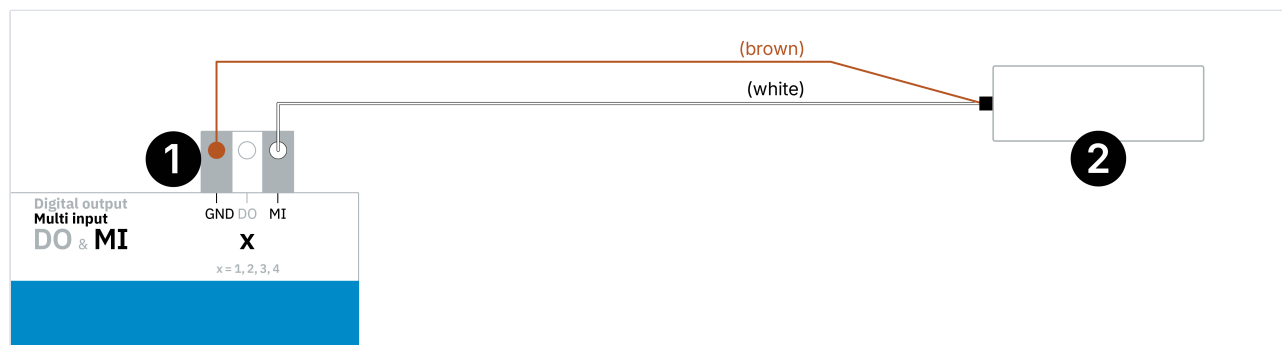
PT1000 adhesive sensor: Sensor connection
