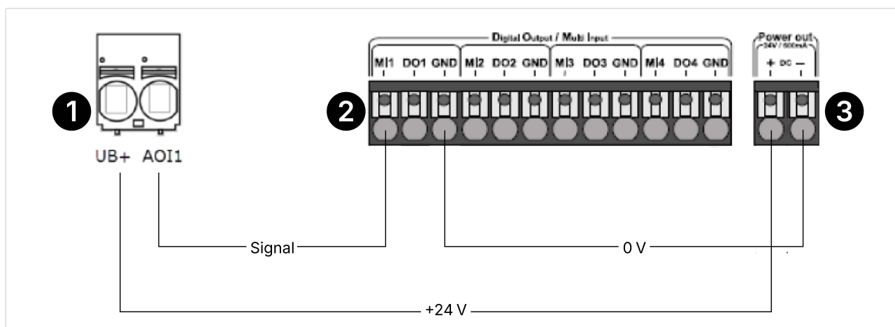
Thermokon AGS55+ ambient temperature sensor: Sensor connection
